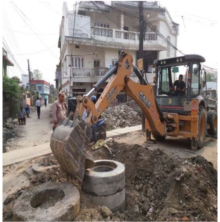
Precast Manhole Installation
